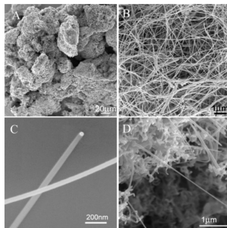
Figure 1. (A–C) SEM images of Ge nanowires made from \text{GeI}_2 in TOP at 350^\circ\text{C} with Bi nanocrystals as growth seeds ( \text{GeI}_2 :Bi = 80:1 n:n). SEM reveals a high yield of high quality Ge nanowires with an average diameter of 50\text{ nm} . (C) A representative Ge nanowire shows a Bi nanoparticle at its tip. (D) Ge nanowires synthesized at a lower mole ratio of \text{GeI}_2 to Bi of 50:1 (n:n) were of lower quality.
